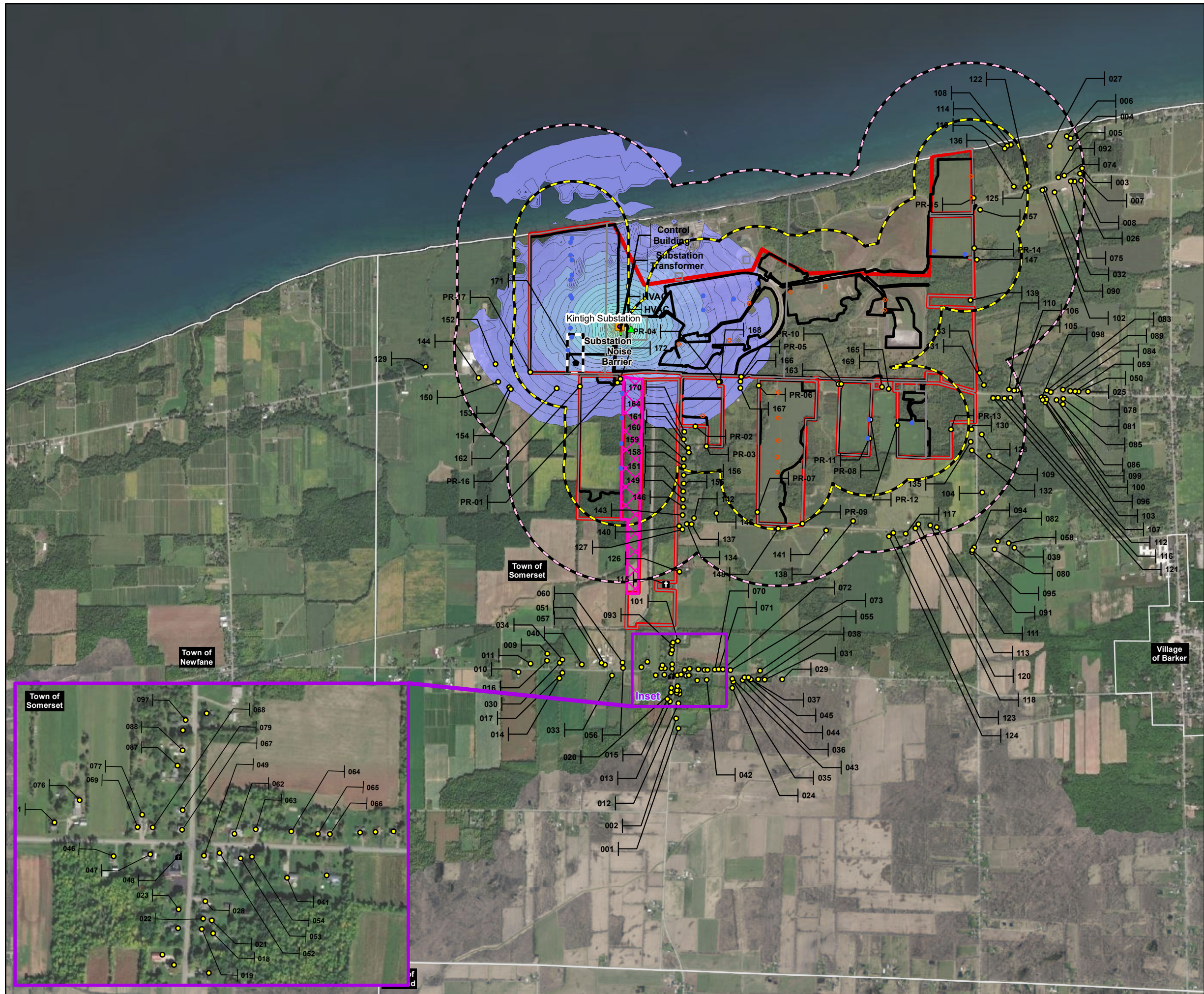
Figure 7-2 Mitigated Substation Only Sound Levels, (dBA) Somerset Solar Niagara County, NY March 2023
