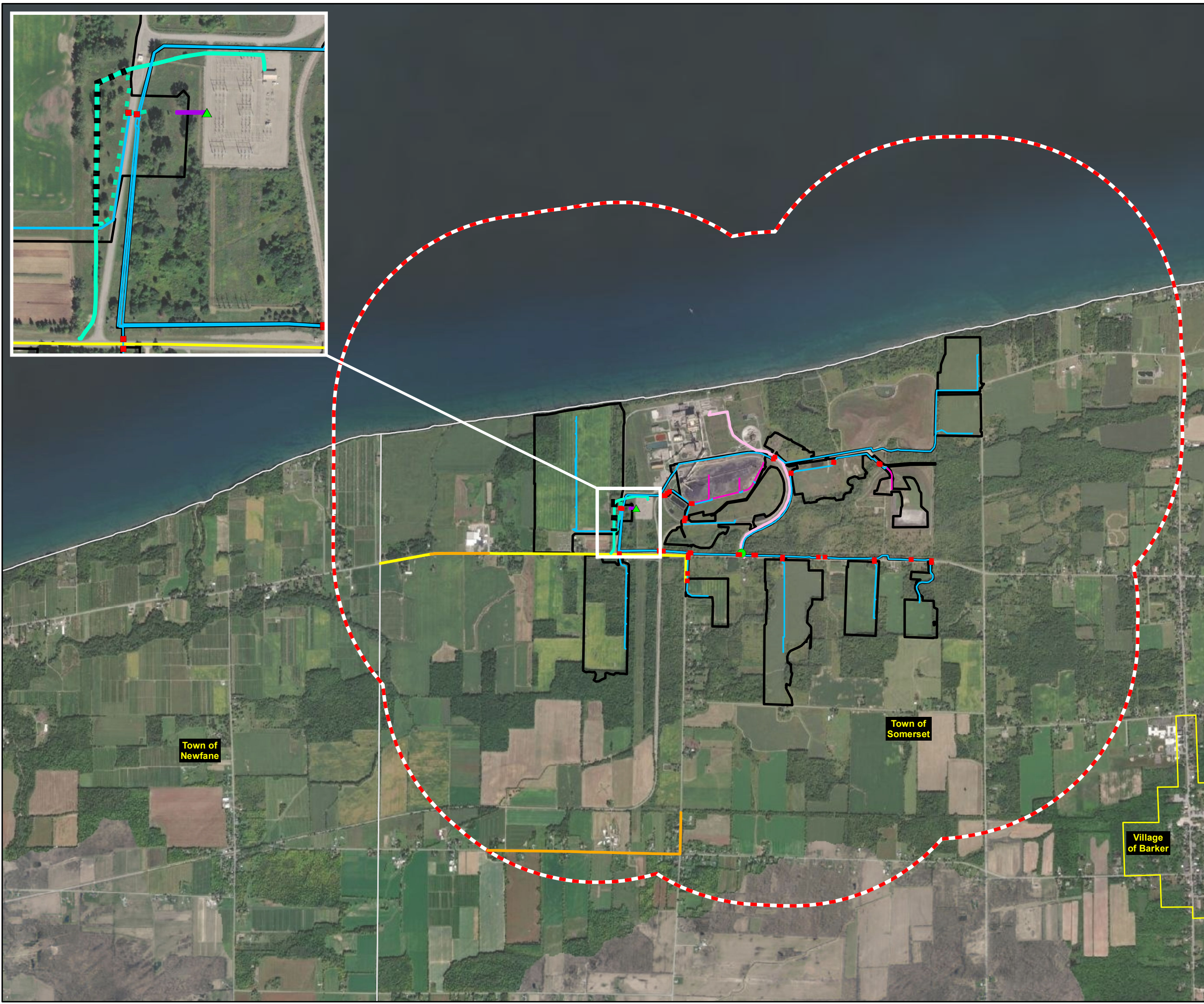
Figure 20-1 Underground Cables, Fiber Optic Cables and Telecommunication Poles Somerset Solar Niagara County, NY March 2023
