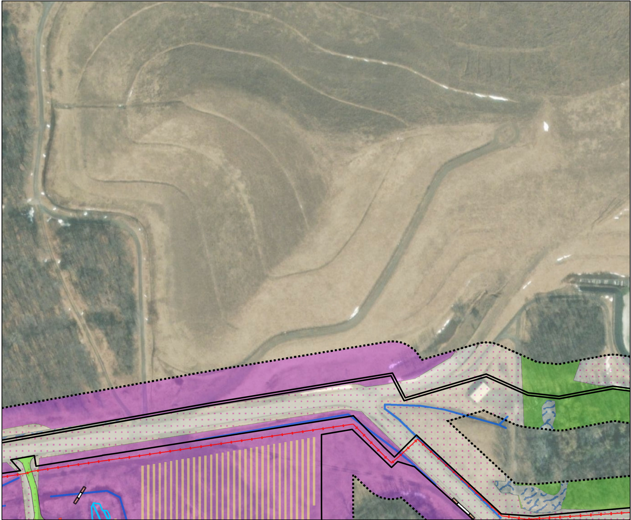
Figure 11-1 Map 12 Change in Plant Communities in Facility Site Somerset Solar Niagara County, NY March 2023
