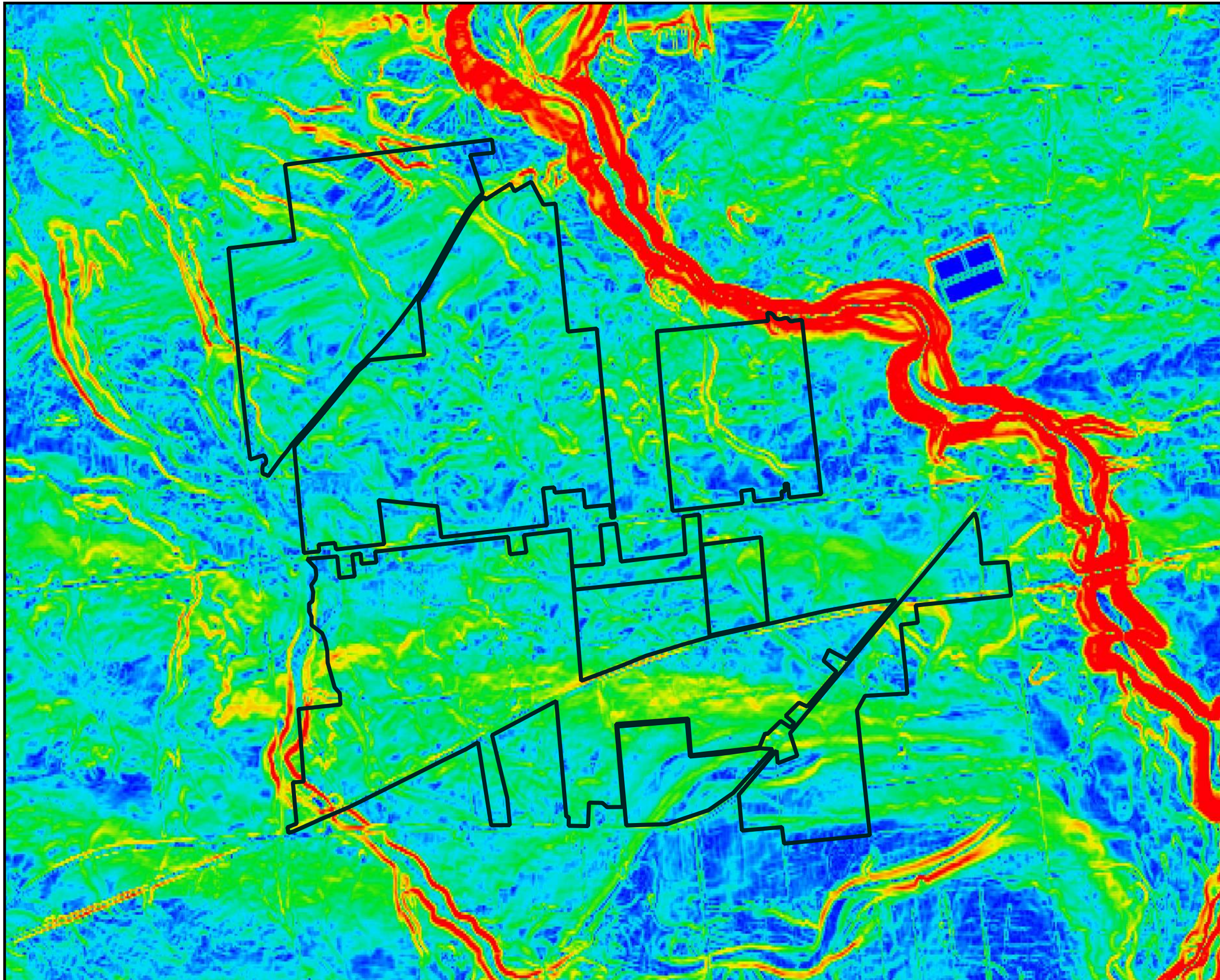
FIGURE 10-1 SLOPE MAP
