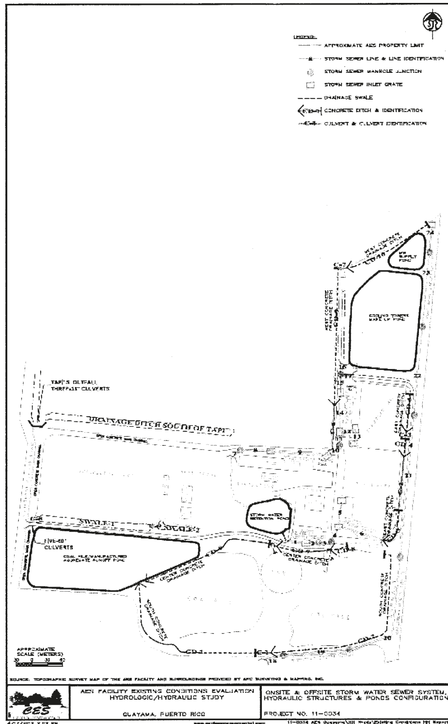
Figure 3: Onsite and offsite storm water sewer system, hydraulic structures and ponds configuration
