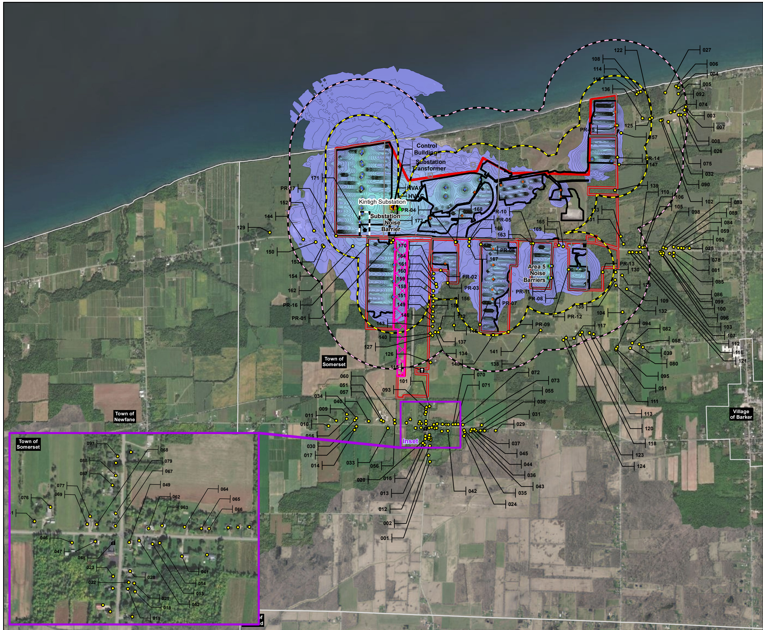
Figure 7-1 Mitigated Full Operational Sound Levels, (dBA) Somerset Solar Niagara County, NY March 2023
