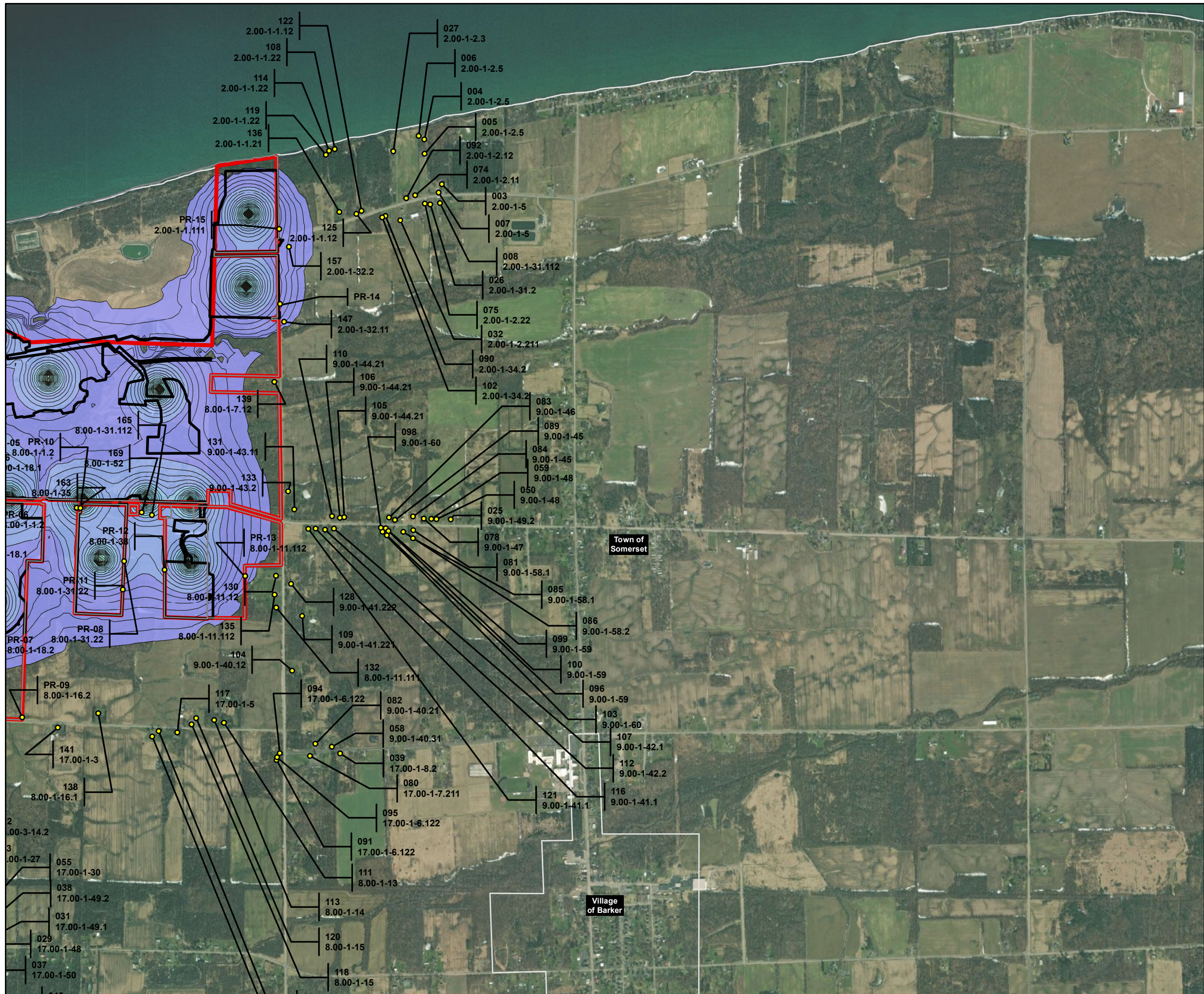
Figure 21B Commissioning Construction Sound Levels, (dBA) Somerset Solar Niagara County, NY March 2023
