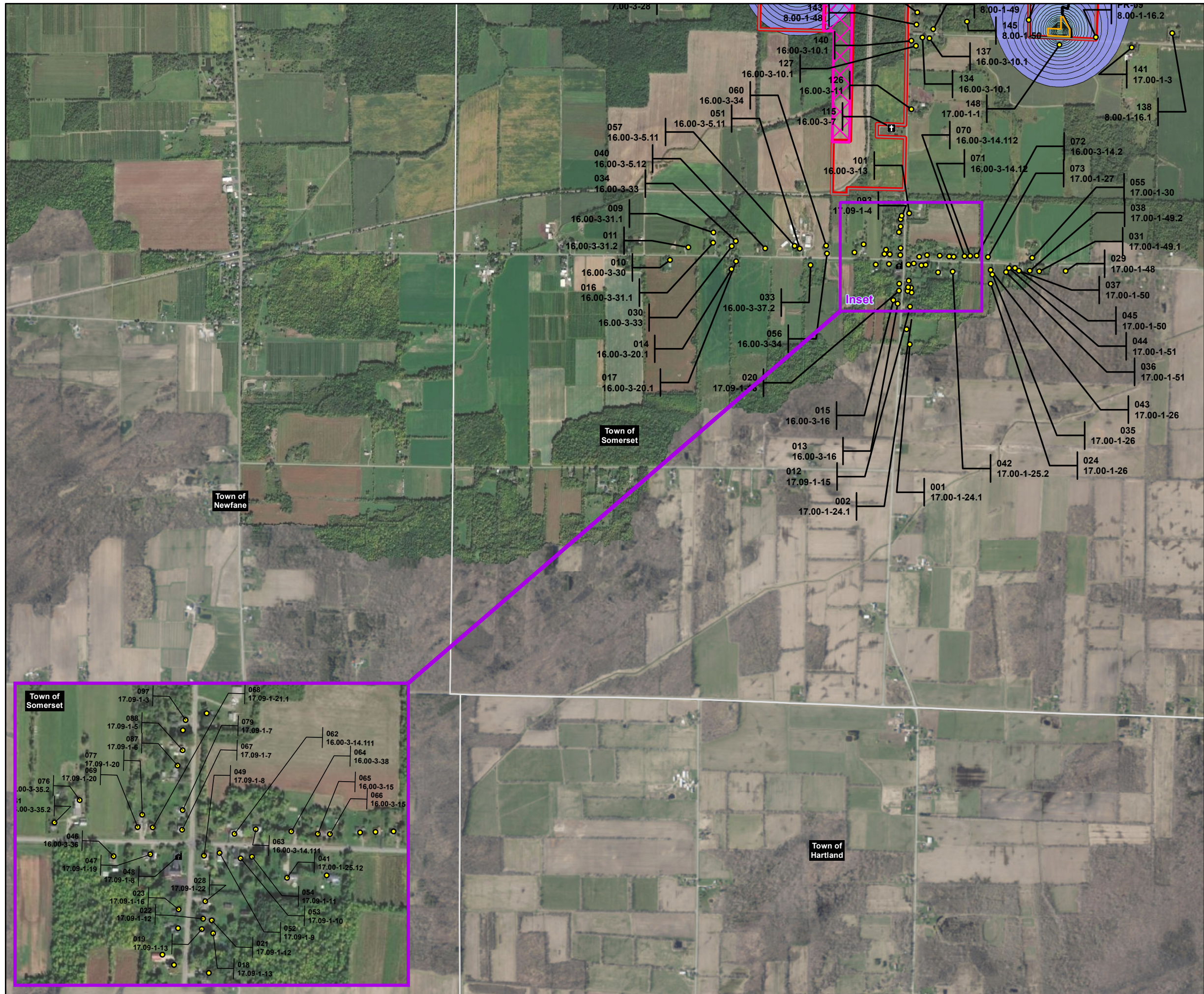
Figure 22C Laydown Areas Construction Sound Levels, (dBA) Somerset Solar Niagara County, NY March 2023
