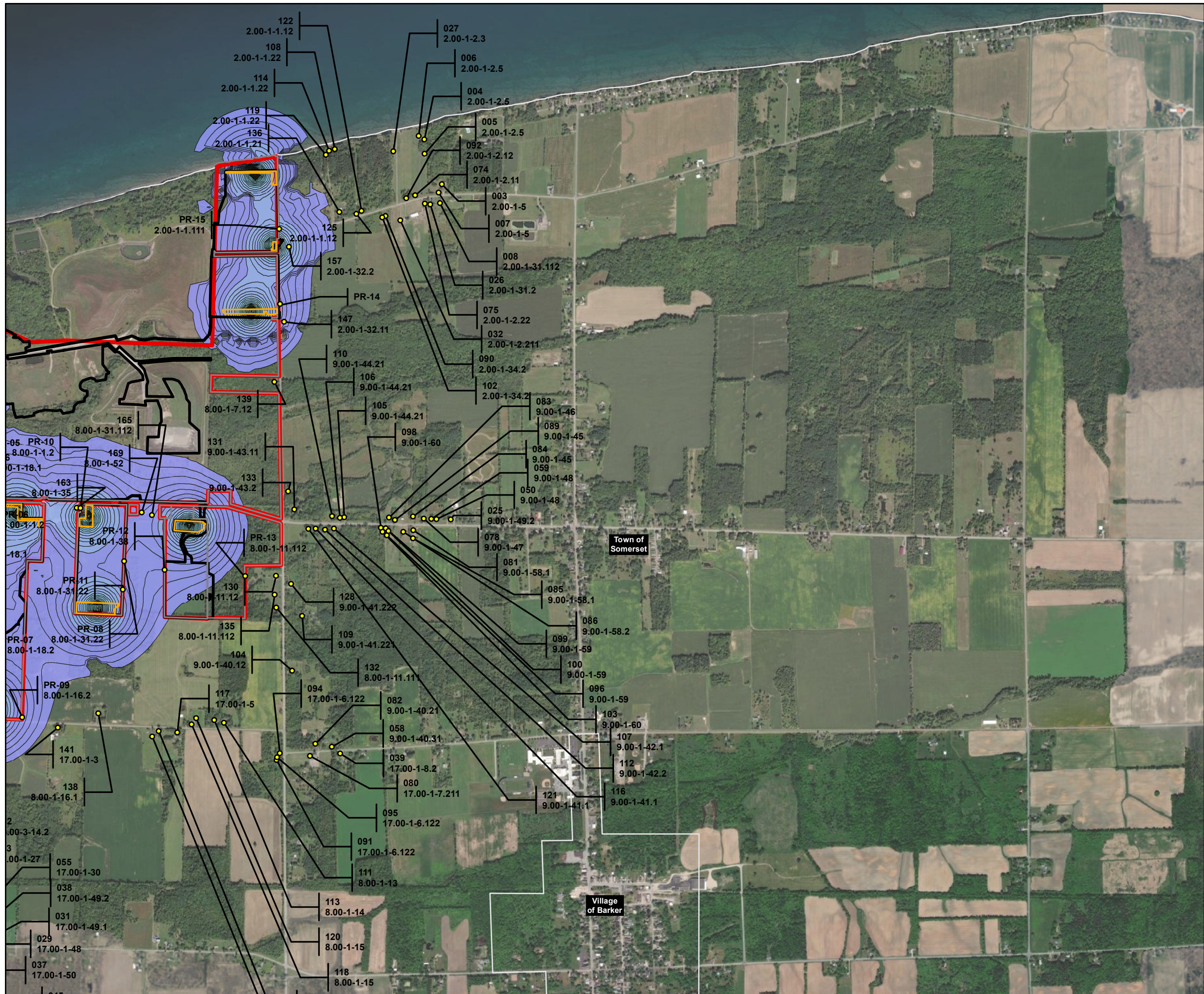
Figure 22B Laydown Areas Construction Sound Levels, (dBA) Somerset Solar Niagara County, NY March 2023
