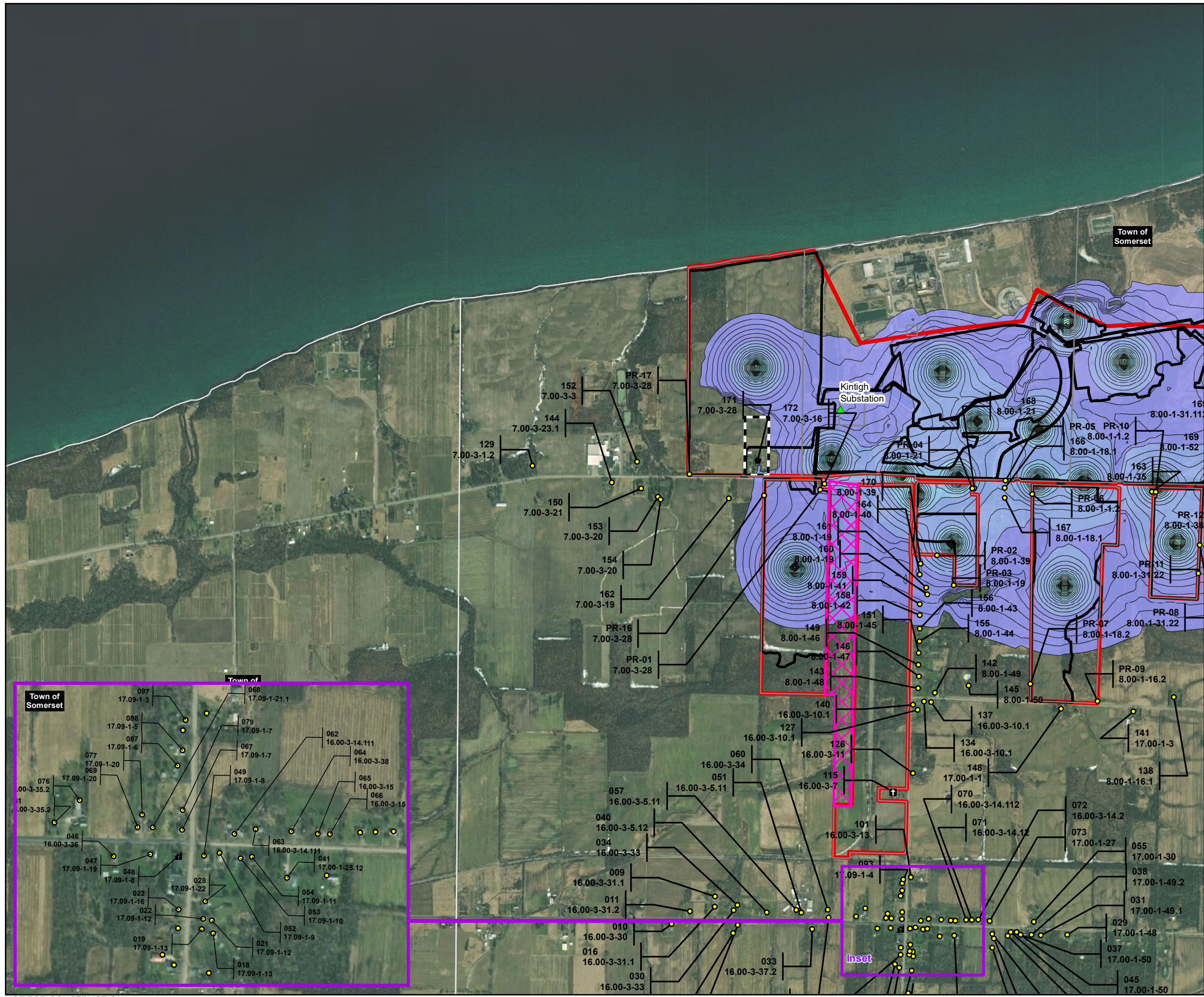
Figure 21A Commissioning Construction Sound Levels, (dBA) Somerset Solar Niagara County, NY March 2023
